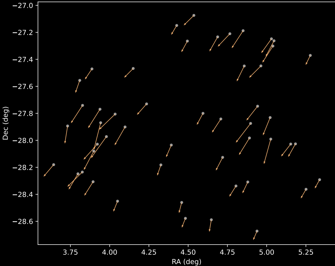
APOGEE DR17 Cluster 3 Proper Motion Vectors (n=50)
