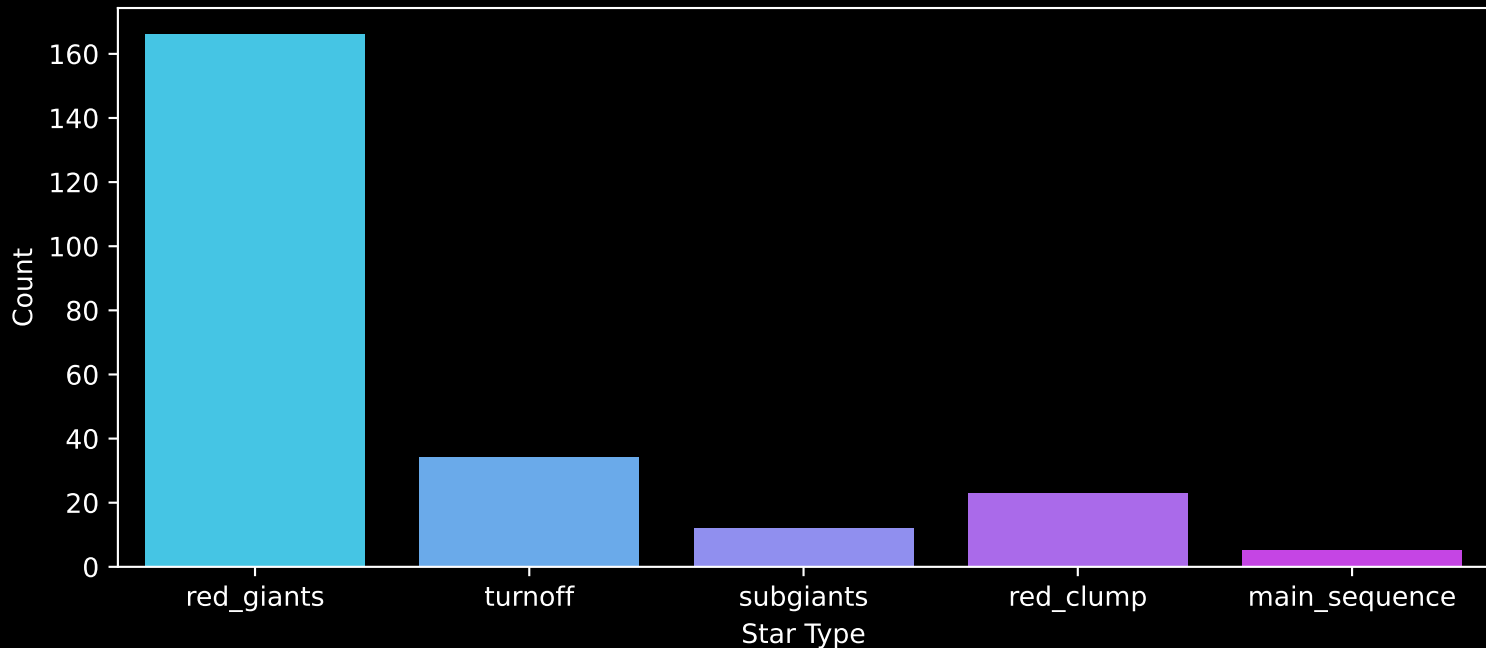
APOGEE DR17 Field: [000+02] Count plot of Star Type
