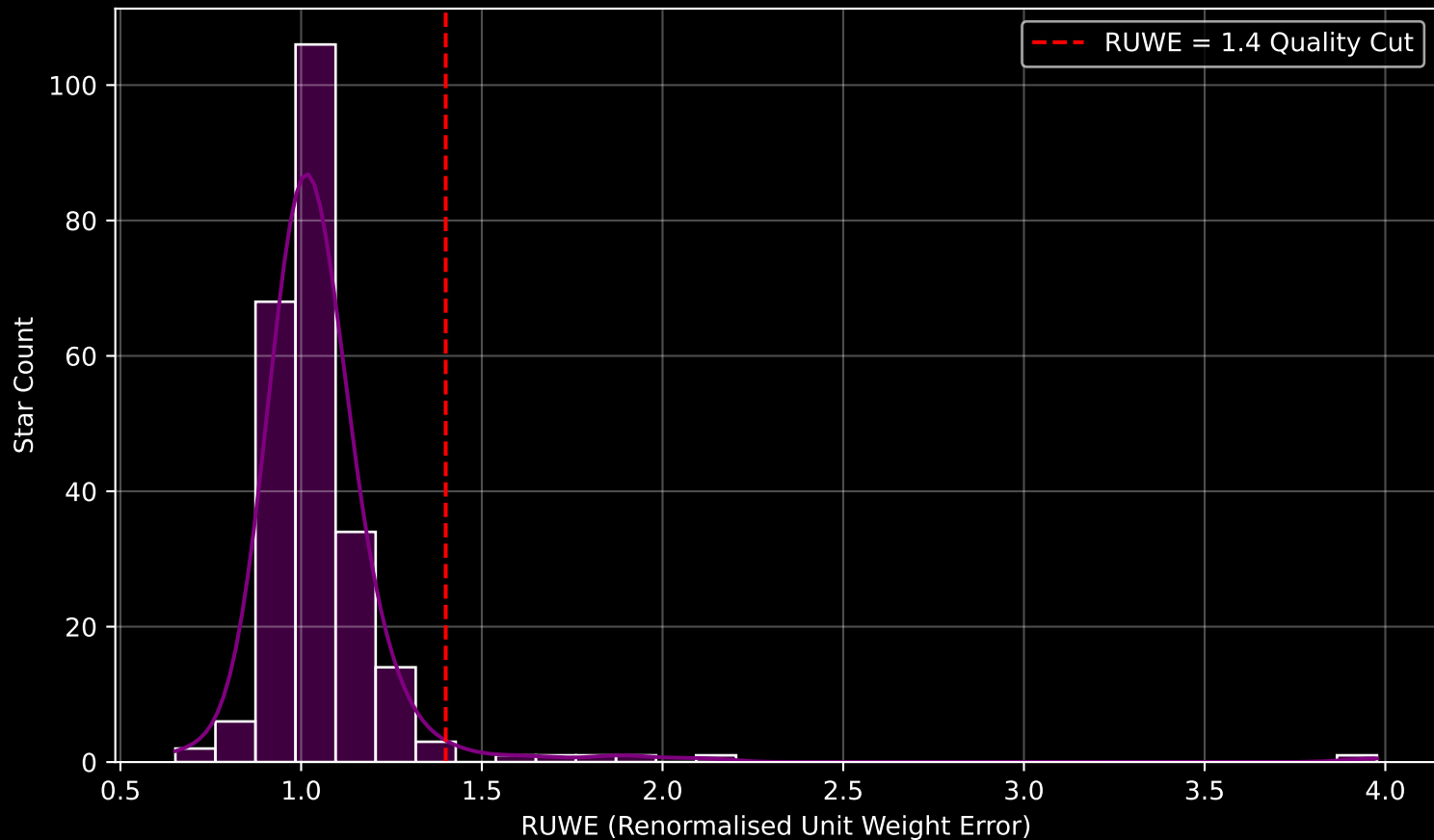
GAPOGEE DR17 Field [000+02] RUWE Distribution (n= 239)
