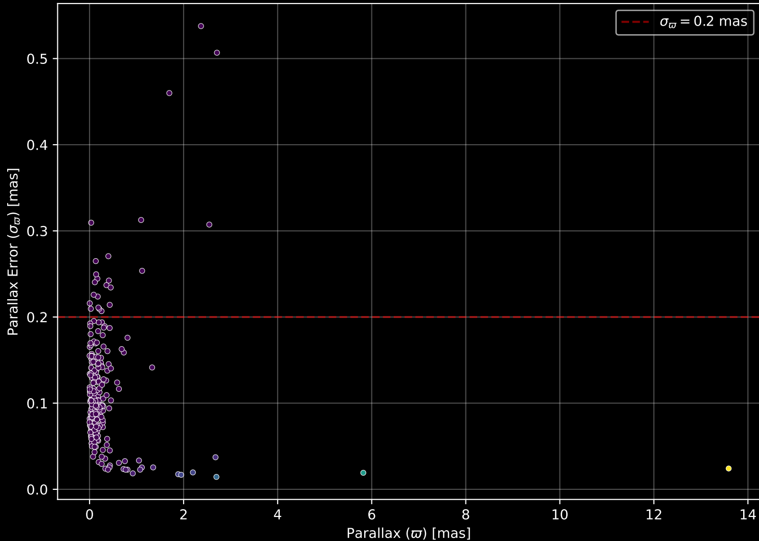
APOGEE DR17 Field: [000+02] Parallax Quality (n= 240)
