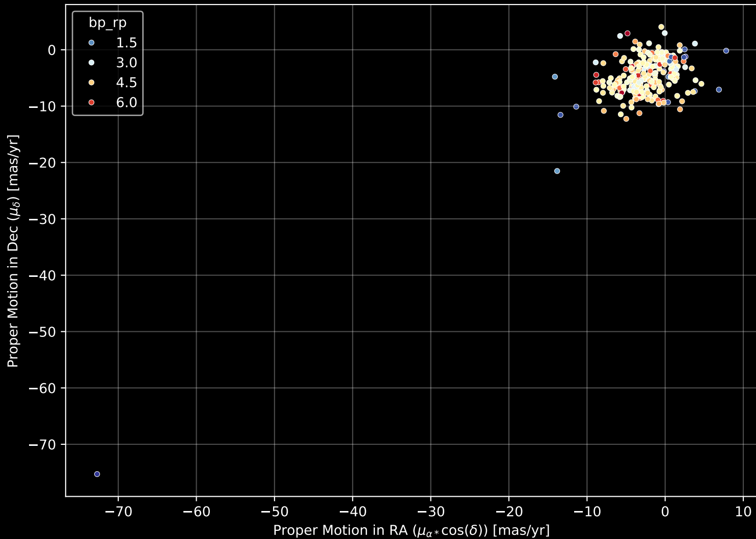
APOGEE DR17 Field: [000+02] Proper Motion Diagram (n= 240)
