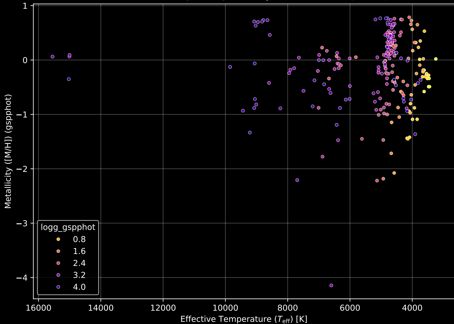
APOGEE DR17 Field: [000+02] Stellar Population Parameters (n= 240)
