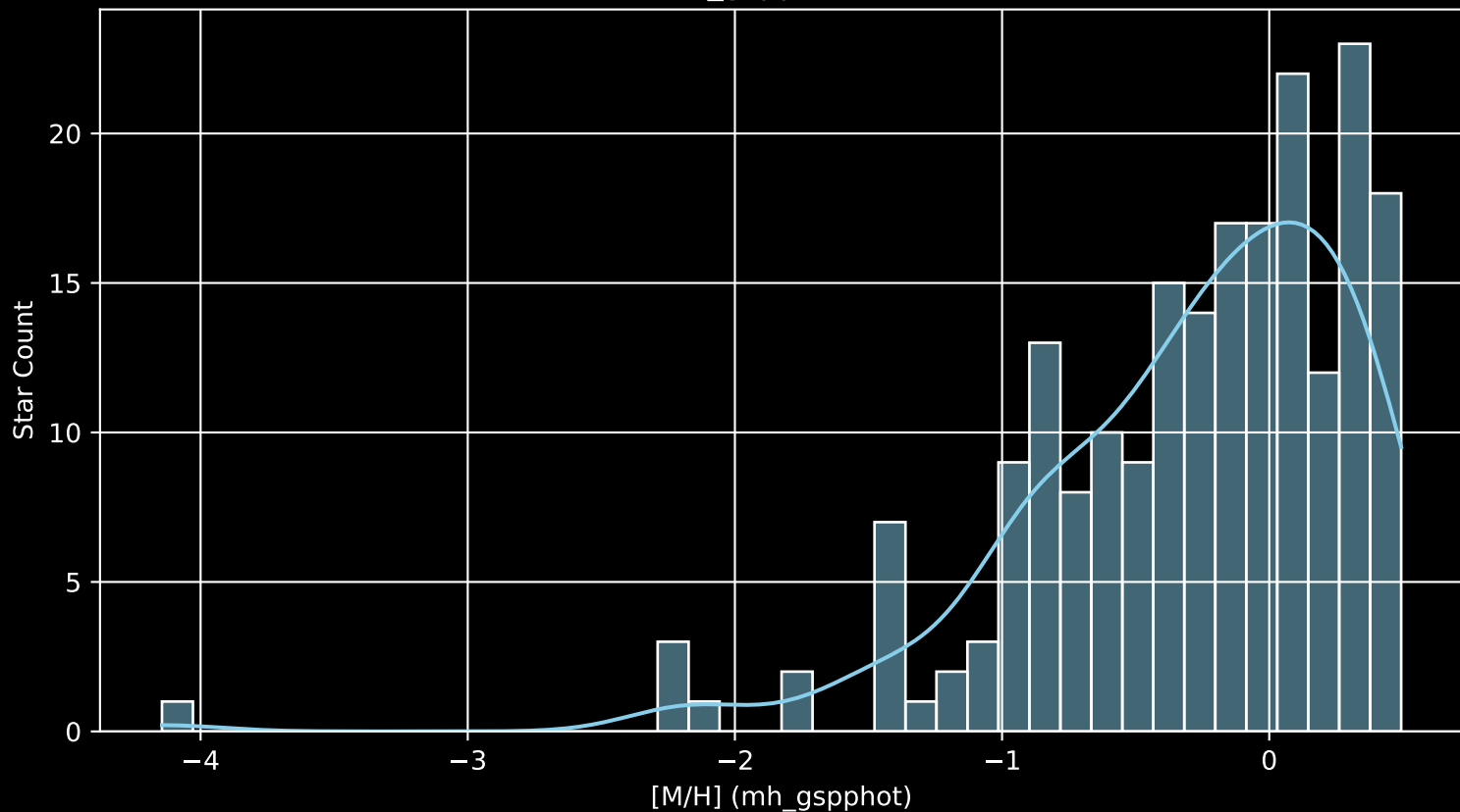
APOGEE DR17 Field: [000+02 [M/H] (mh_gspphot) (n= 207)
